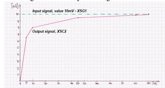
Fig.13. The graph of the output signal level according to the light intensity (applied to the phototransistor) .
