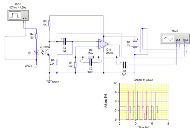
Fig.16. The circuit diagram of a circuit that shows the arterial impulse.
