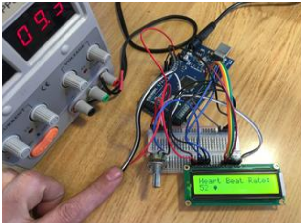
Fig.24. Digital photoplethysmograph with the XD-58C pulse sensor connected to a ArduinoMega 2560 motherboard 12 .
