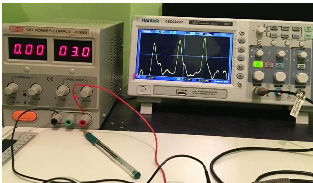
Fig.19. The waveform of arterial pulse using the XD-58C pulse sensor connected to an oscilloscope.
