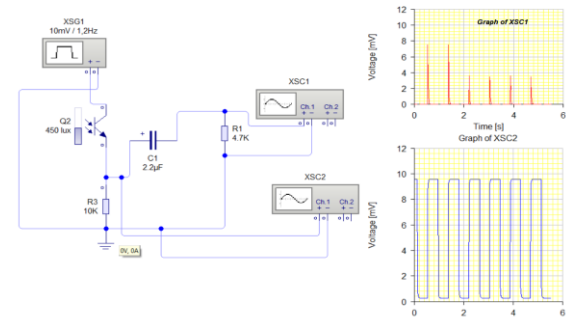
Fig.11. Light intensity has 450 lux, output signal is 9 mV.
