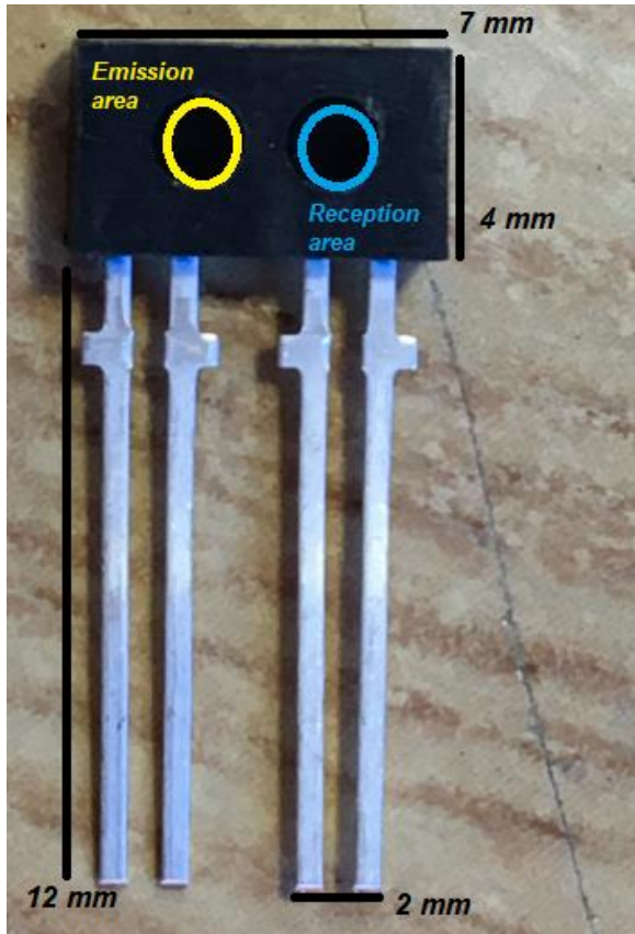
Fig.14. The TCRT1000 reflexiv photoelectric transducer.
